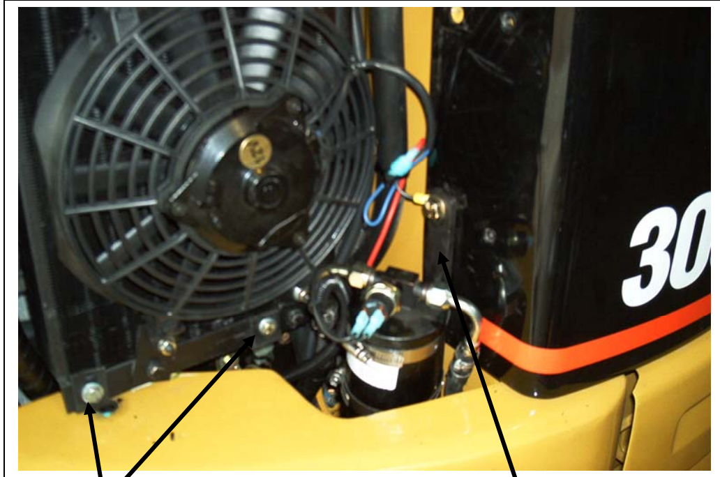
Condenser sits into these two lower brackets.
