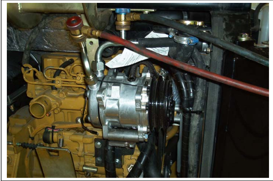
Compressor and mount installed.
