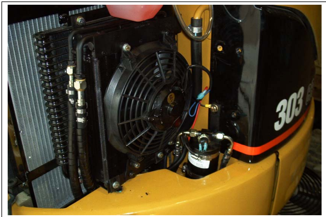
Condenser upper bolting locations.
