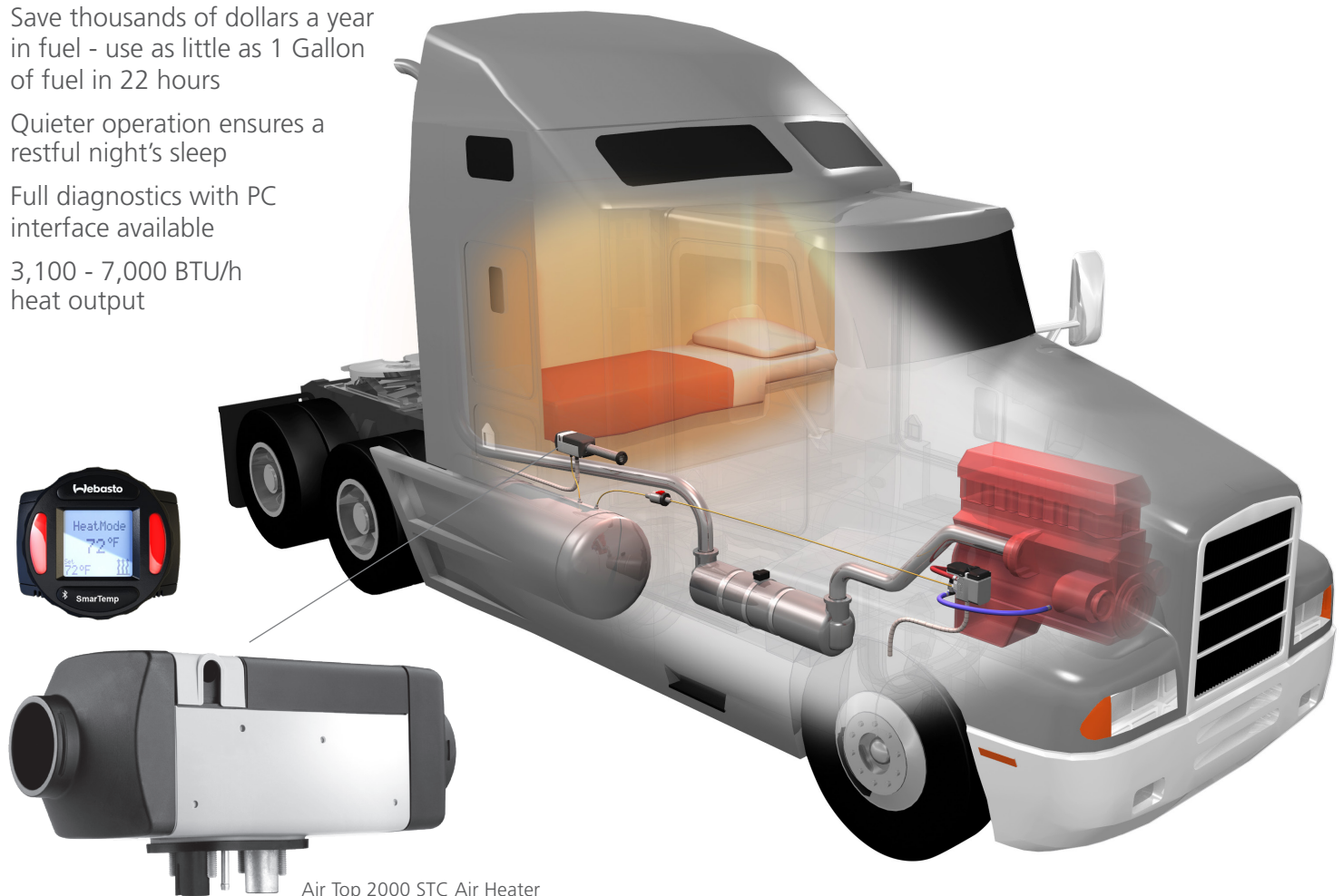
Air Top 2000 STC Air Heater with SmarTemp Control 3.0 Bluetooth (Precision Bunk Temperature Management with Programmable Heater Start Time)
